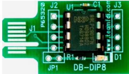
Board Dimensions 1.218" x 0.7"
