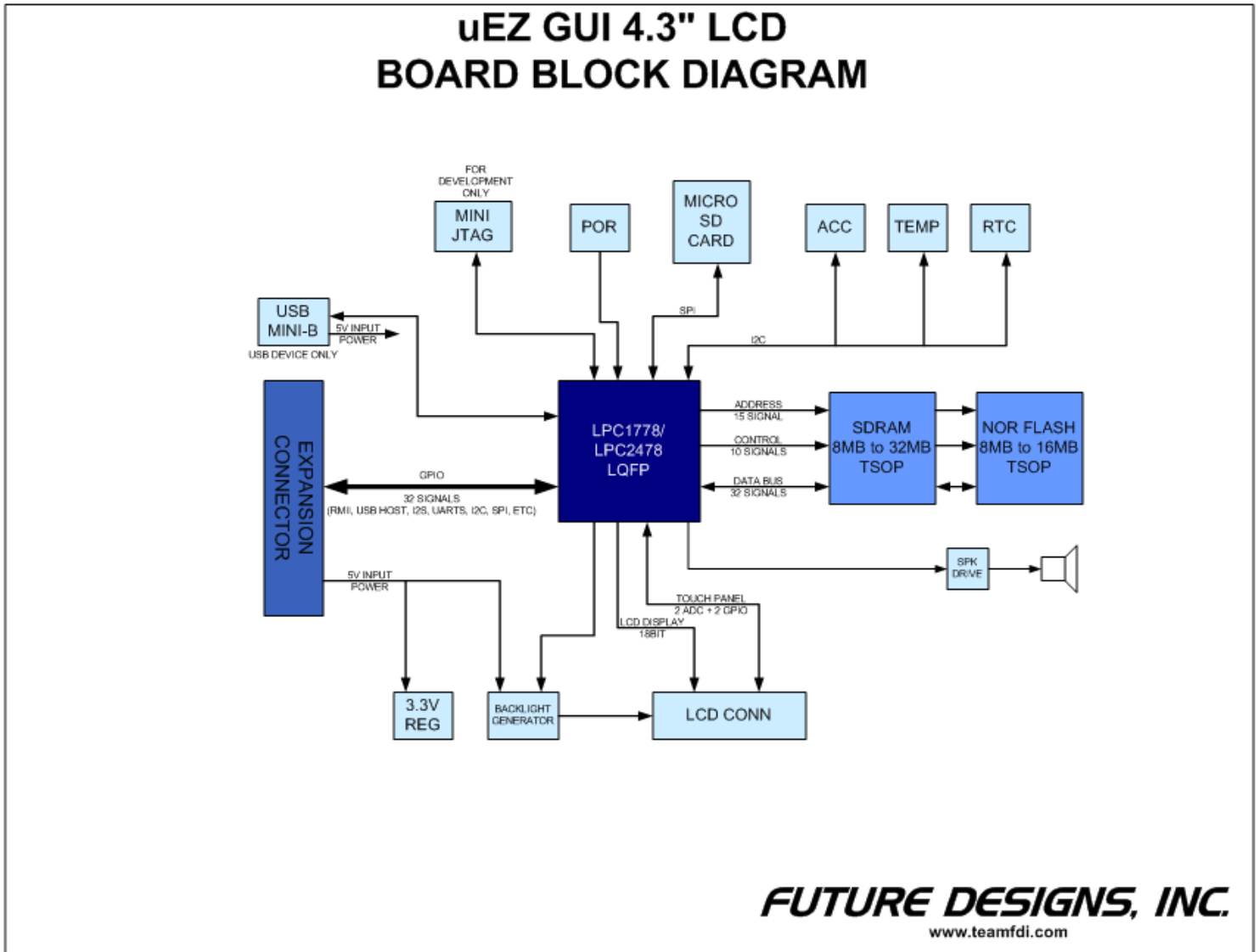
Figure 1 – uEZGUI-xxxx-43WQS Block Diagram
