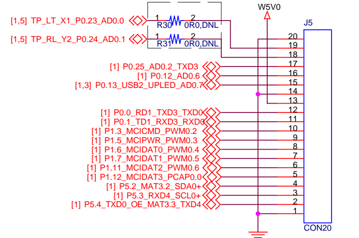
SECONDARY EXPANSION CONNECTOR
